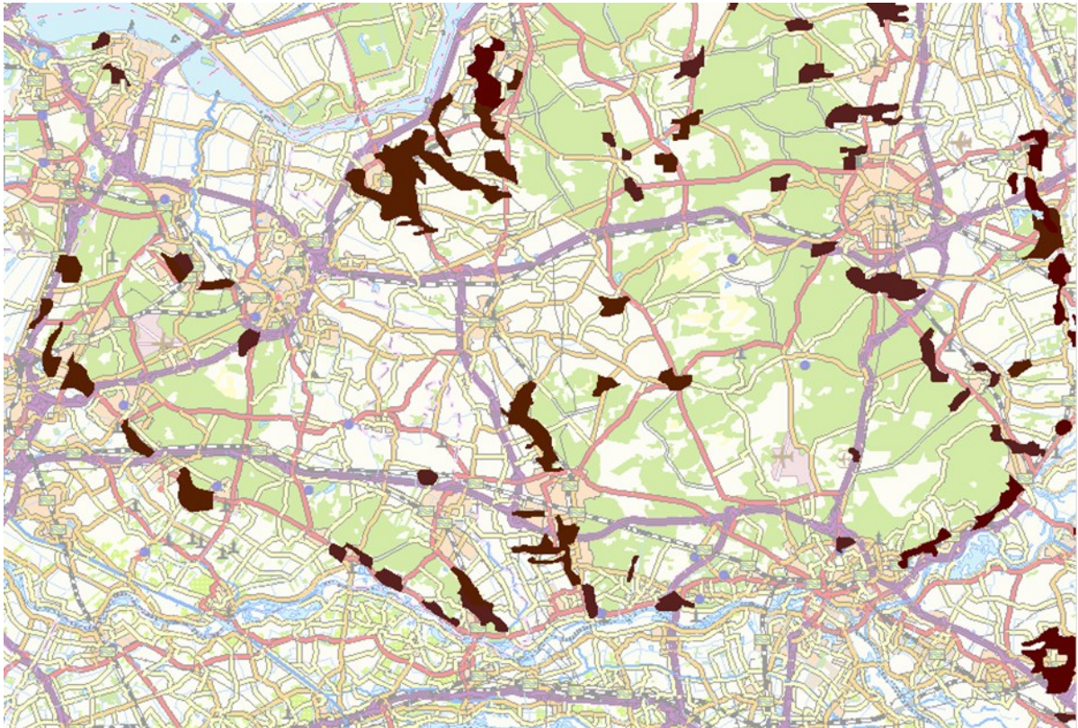
Anthropogenic soils around Wageningen
