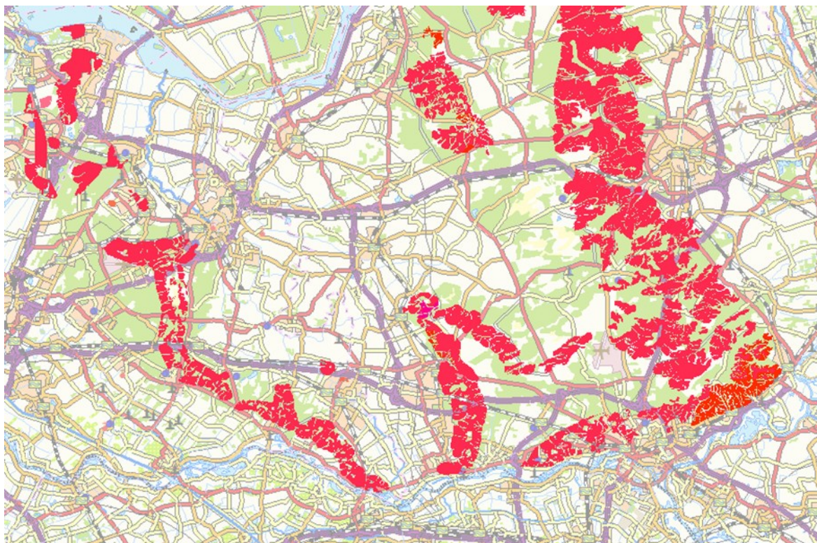
The location of the pushed moraines in the landscape around Wageningen
